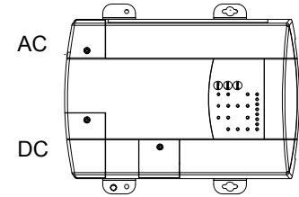
Figure 5 Mounting Orientations (Deck and Horizontal)
