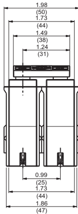
HOM two-pole
