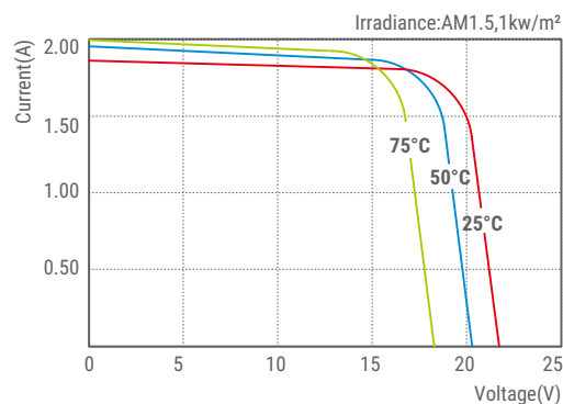
SLP030-12U I-V Curves
