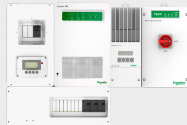
Configuration with SW PDP for 120/240 VAC
